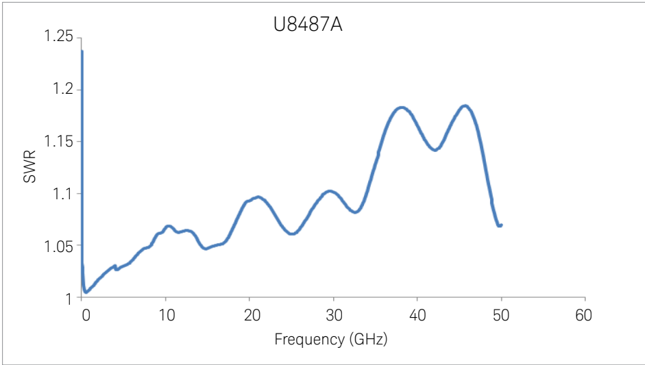
Figure 6. Typical SWR for the AC-coupled U8487A (Option 100)
