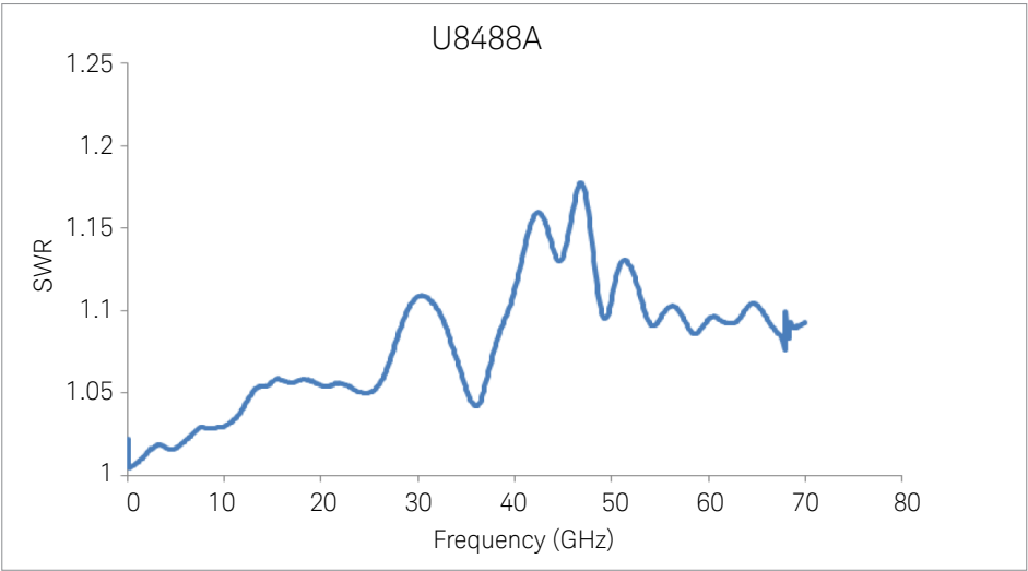
Figure 7. Typical SWR for the AC-coupled U8488A (Option 100)
