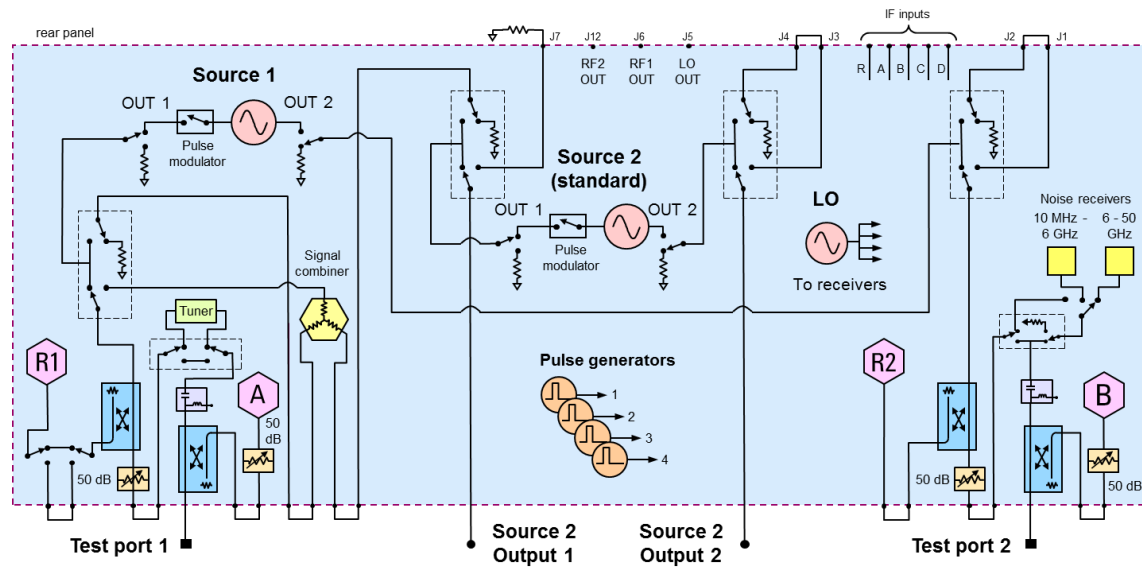
Figure 4. 2-Port N5247B Option 224 with 029
