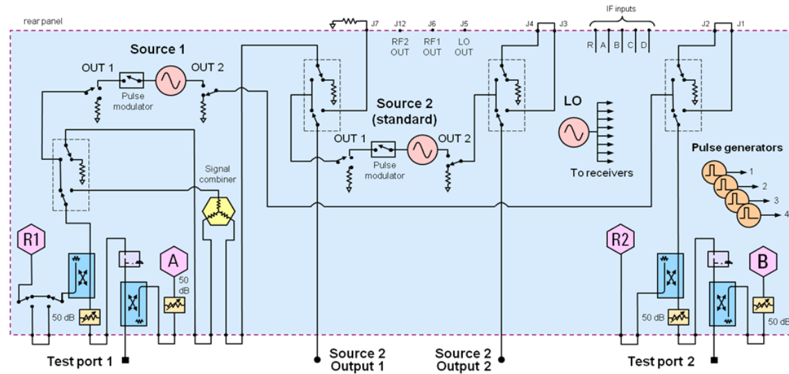
Figure 3. 2-Port N5247B Option 224
