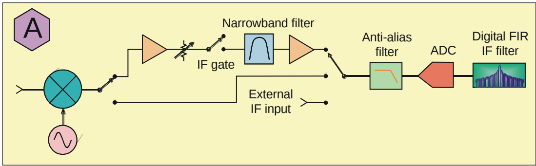
Figure 10. Receiver Block Diagram
